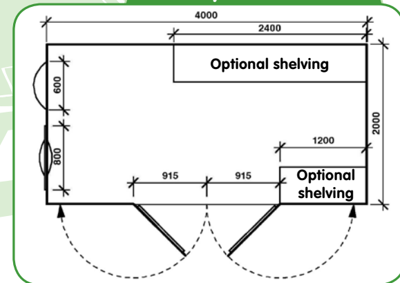
Playcabin Plan
